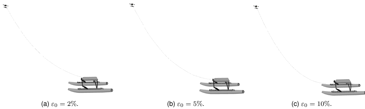
Figure 4.9: Shape of the tether for different slack ratios, displayed in Foxglove.
