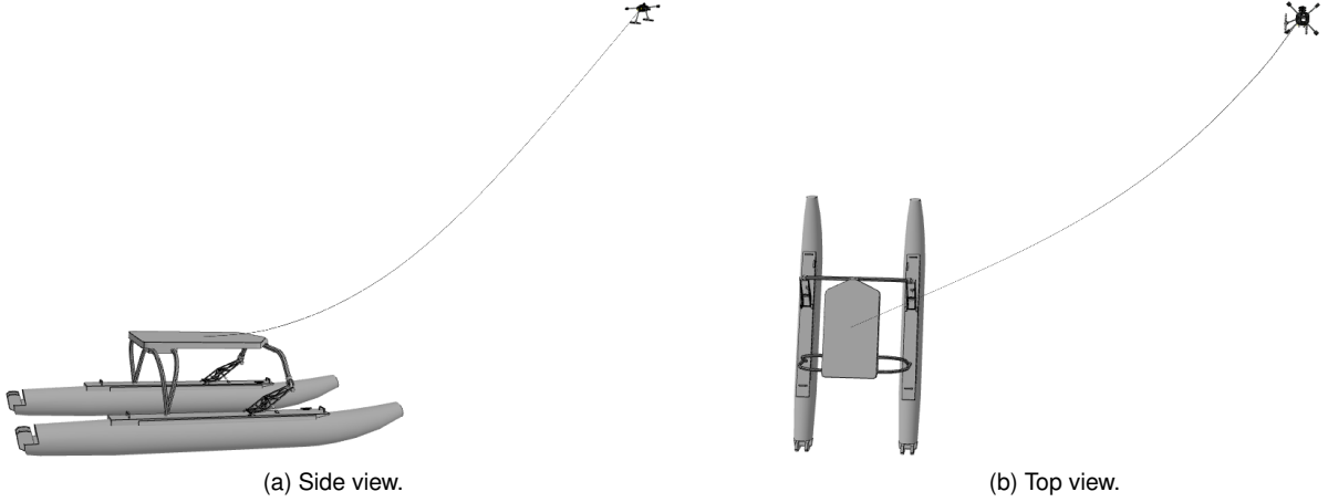
Figure 4.6: The tether between the USV and the UAV, displayed in Foxglove.
