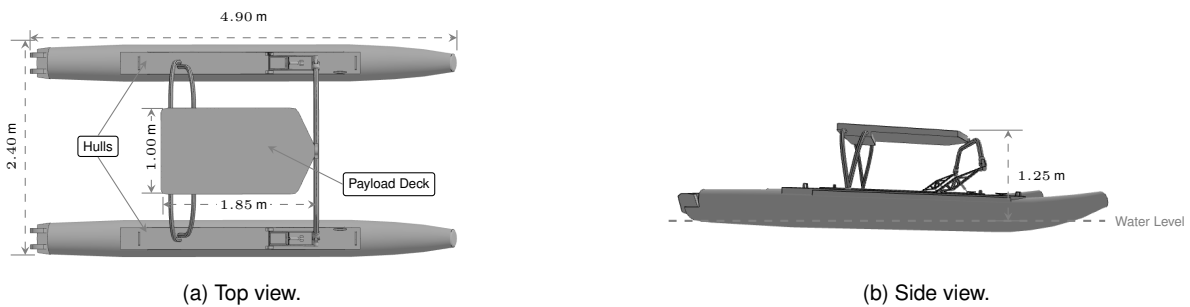
Figure 4.3: WAM-V catamaran layout.
