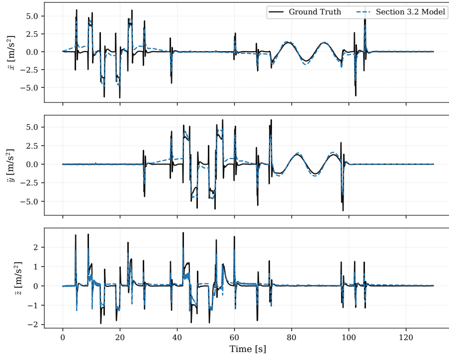
Figure 4.16: UAV inertial acceleration. Ground truth and model driven by the measured attitude.
