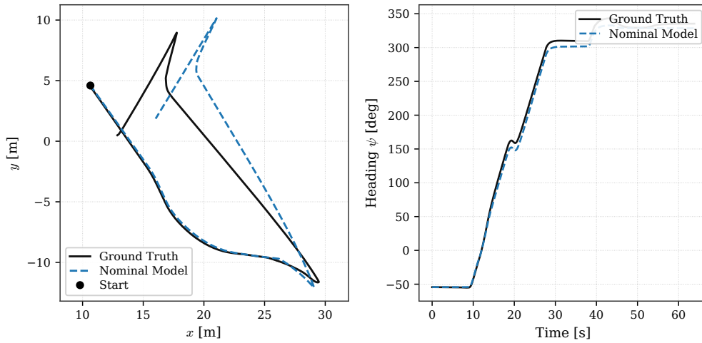
Figure 4.13: USV trajectory and heading validation.
