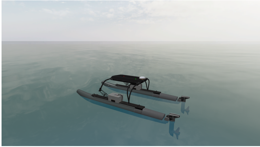
Figure 4.2: The WAM-V catamaran in the simulated world.
