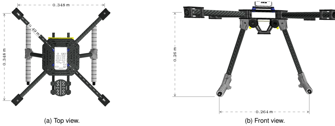
Figure 4.5: x500 quadrotor layout.
