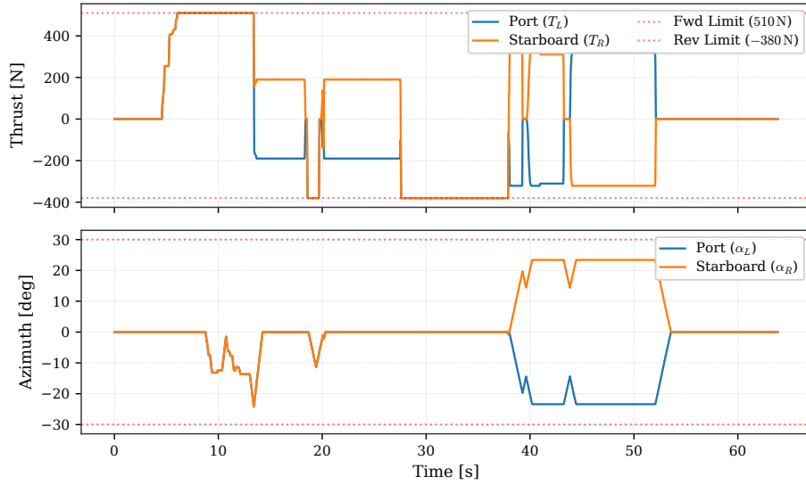
Figure 4.11: USV thruster inputs during the validation maneuver.
