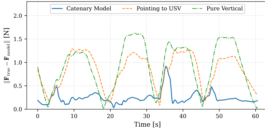
Figure 4.21: Three-dimensional tether force error norm.
