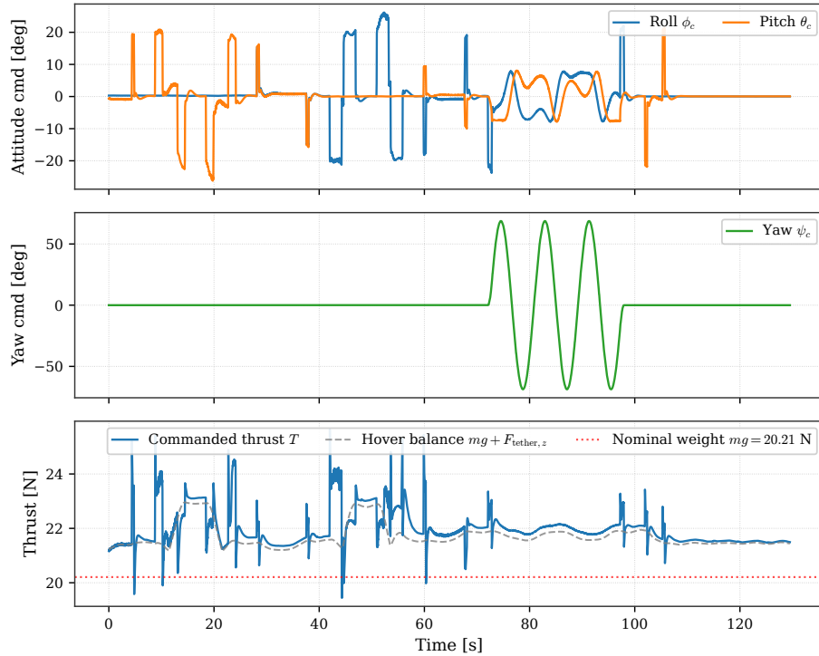
Figure 4.14: UAV attitude and thrust commands during the validation flight.
