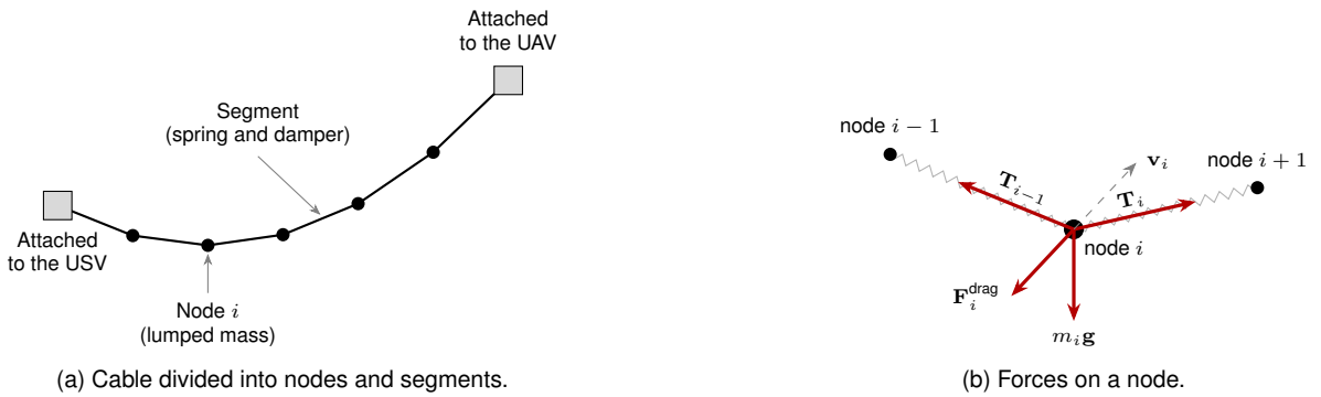
Figure 4.7: Lumped-mass model of the tether. Bending forces are not shown.
