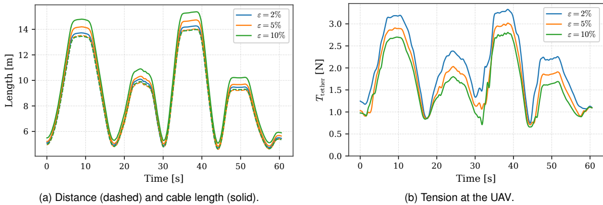
Figure 4.10: Distance between the attachment points, length of the cable, and tension at the UAV for the same trajectory and different slack ratios.
