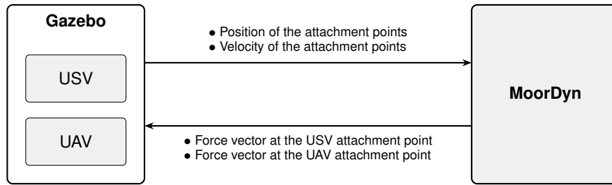
Figure 4.8: Data exchange between the simulation and the tether.
