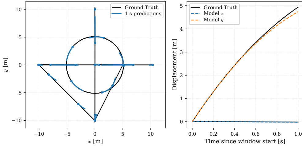
Figure 4.18: One-second open-loop predictions along the flight, and detail of the window with the highest speed.
