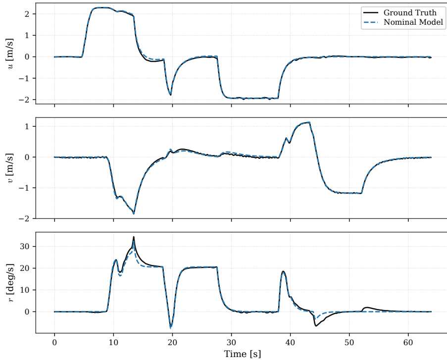
Figure 4.12: USV body-fixed velocities validation.
