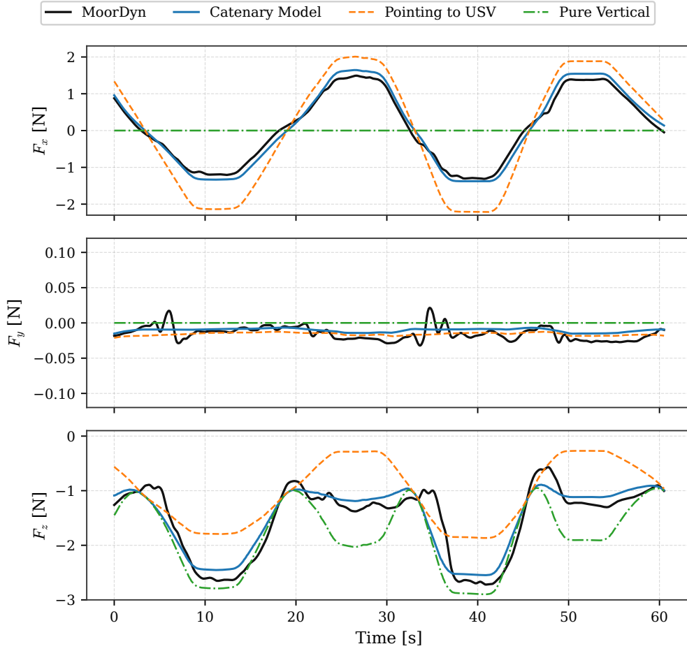
Figure 4.20: Three-dimensional tether force components at the UAV.
