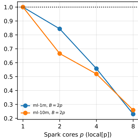
efficiency E(p) = S(p)/p
