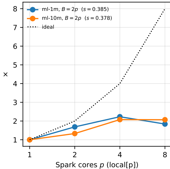
speedup S(p) = T_1/T_p
