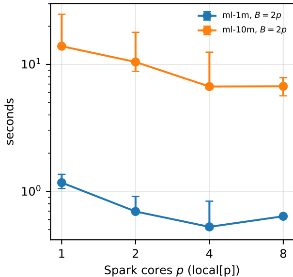
time per iteration
