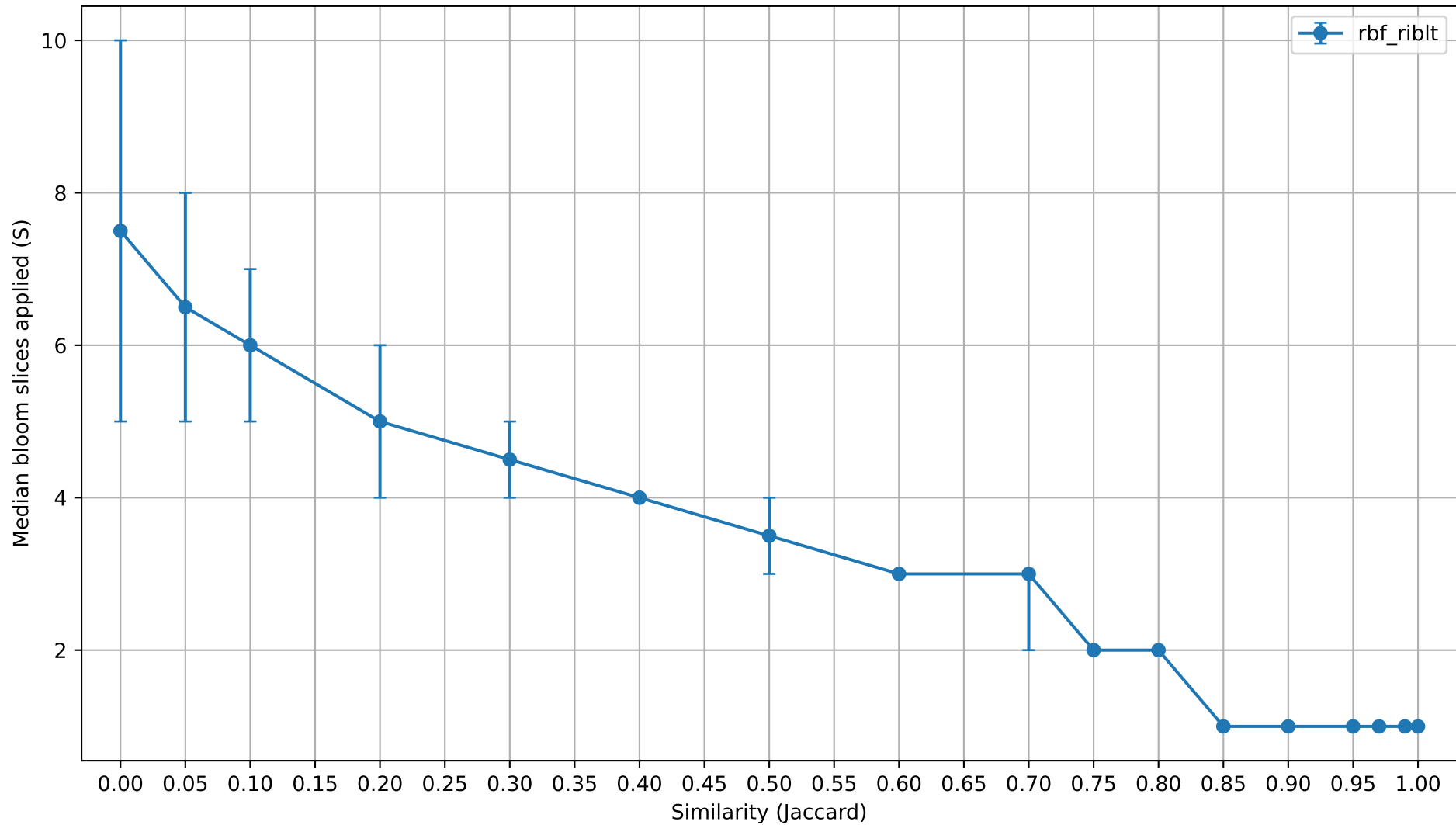
Bloom Slice Count vs Similarity
