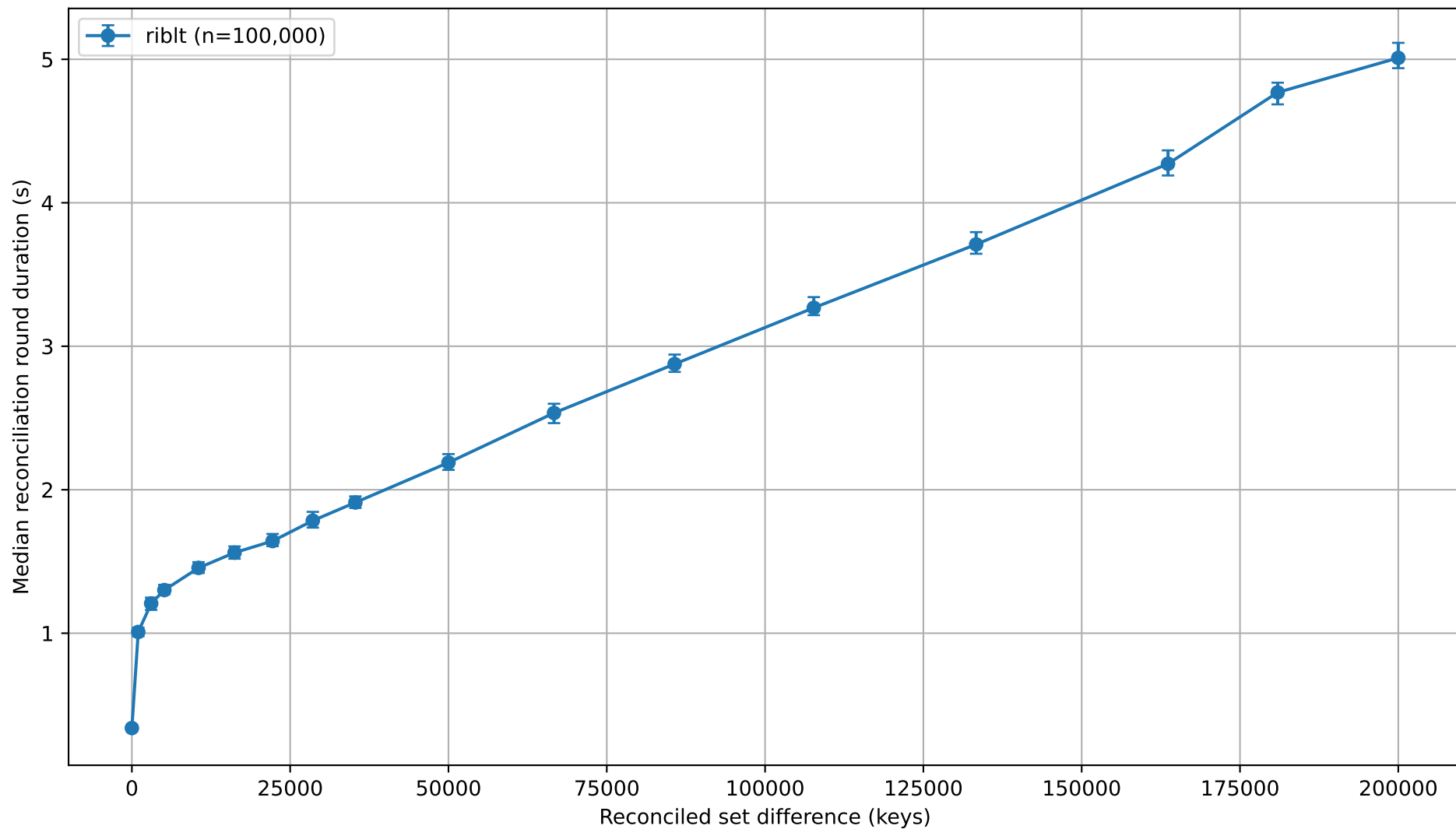
RIBLT round duration vs set difference (fixed set size)
