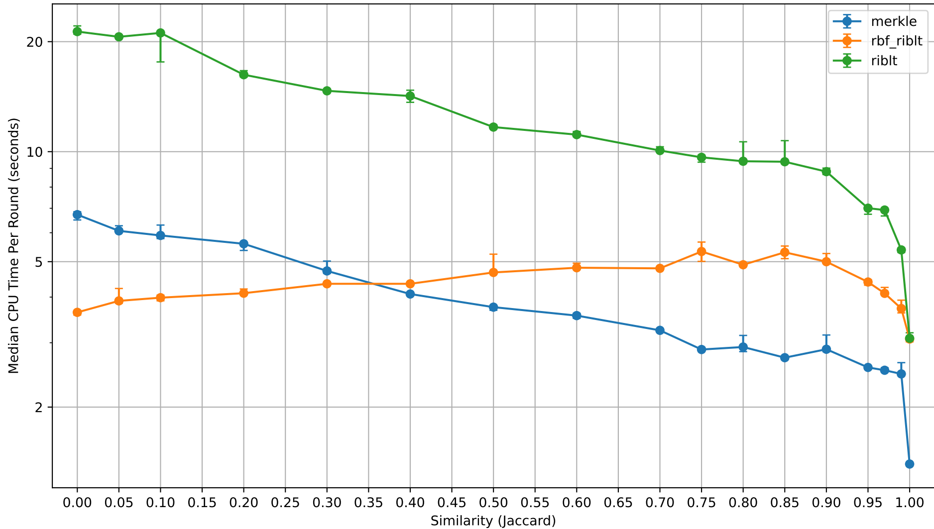
CPU Time Per Round vs Similarity
