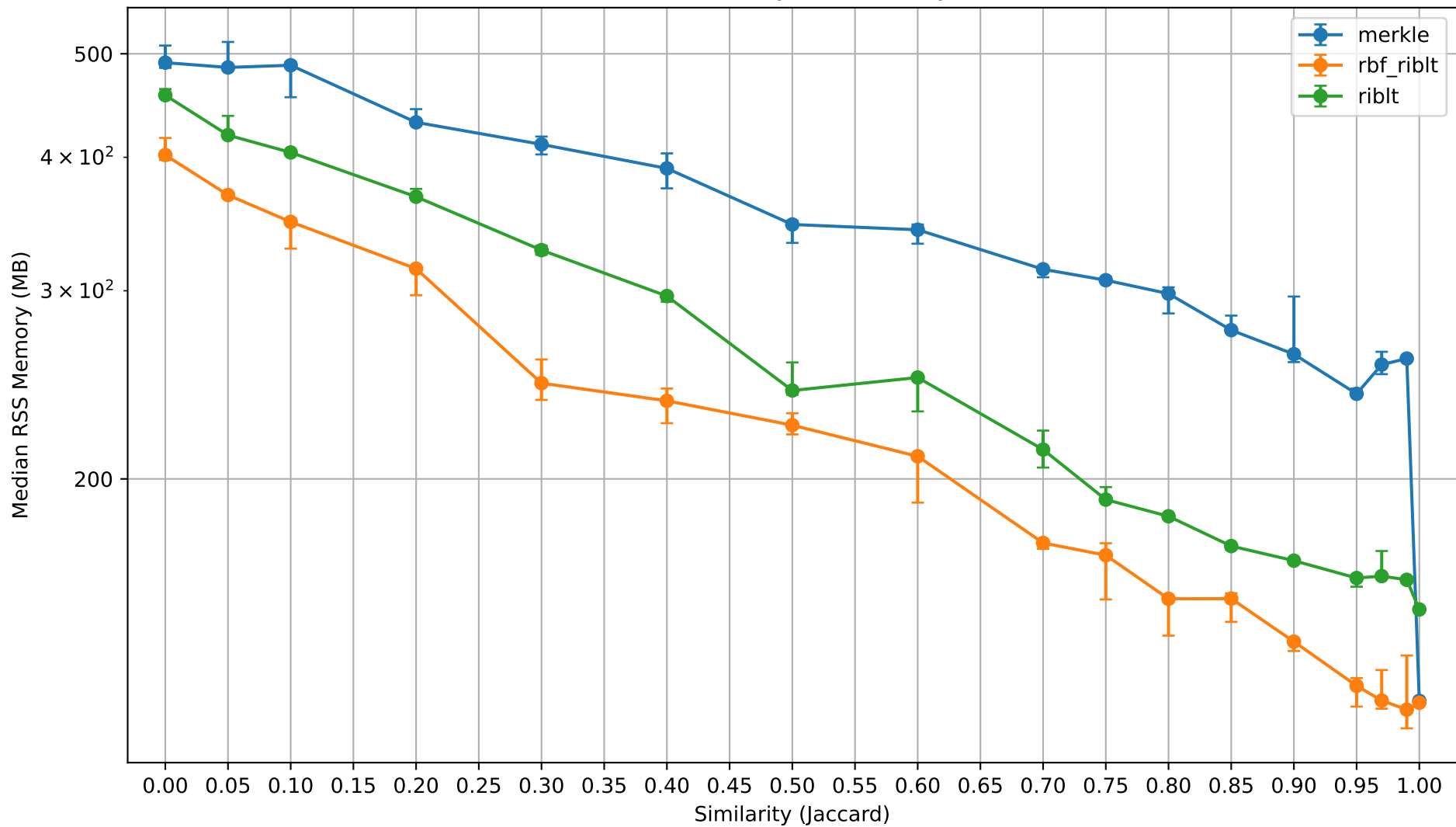
RSS Memory vs Similarity
