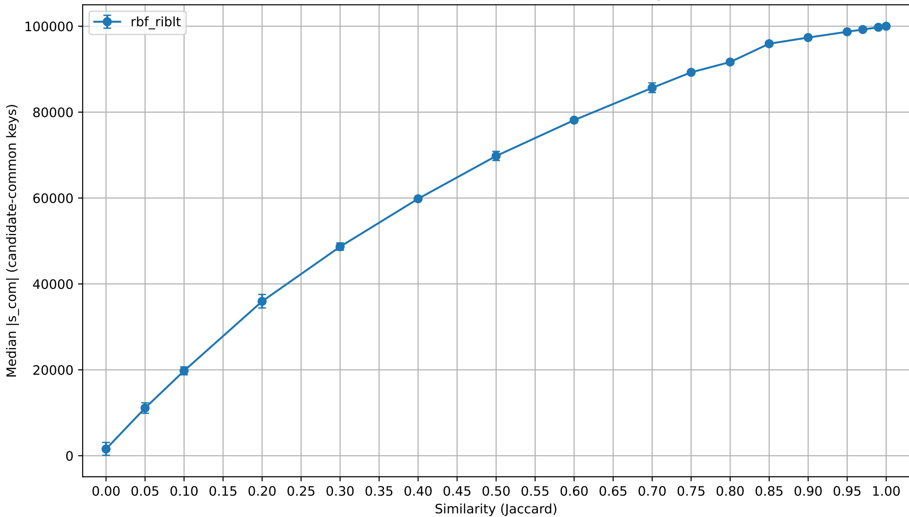
Post-bloom Candidate-Set Size vs Similarity
