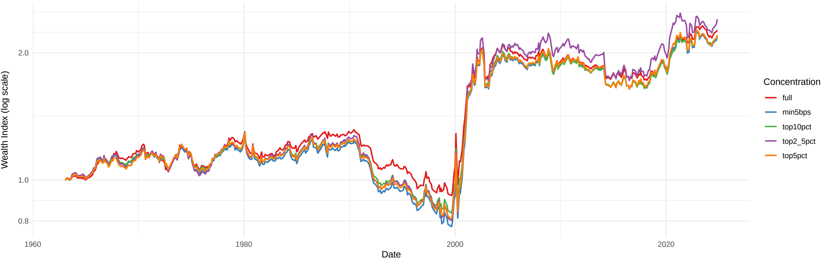
Net Wealth by Concentration Version – CS_LS_50 6M All series: Gross return minus TC + SC + Dividend Tax
