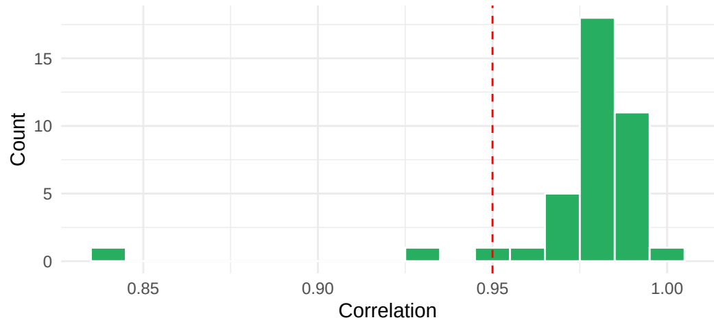
Correlation Distribution
