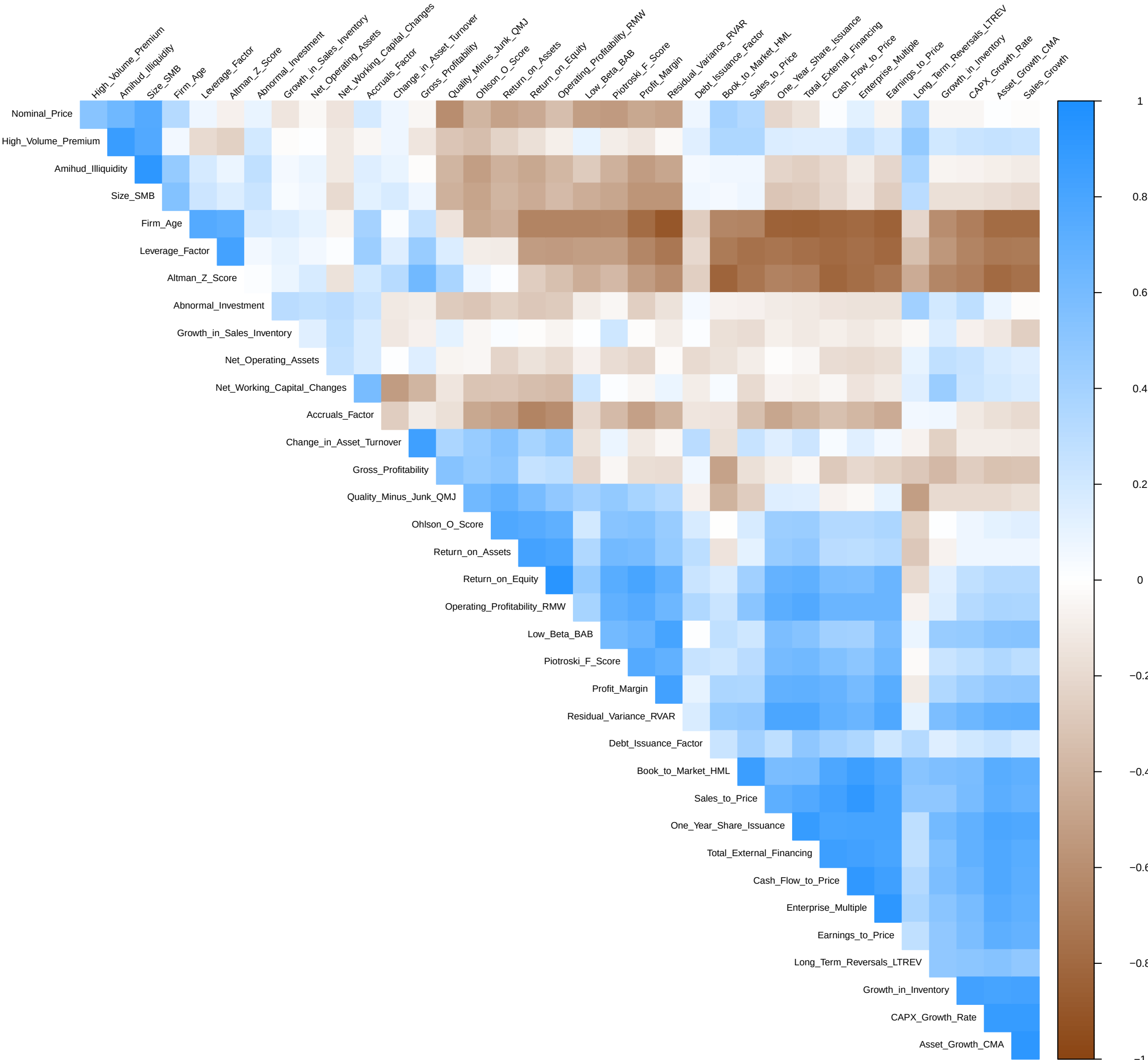
Factor Return Correlation Matrix (Monthly, Hierarchically Ordered)
