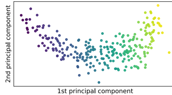
2 components keep 99.8 % of the variance
