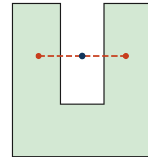
Non-convex set (midpoint outside)
