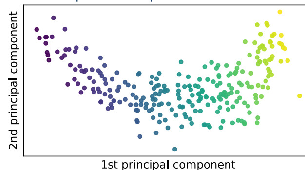
2 components keep 99.8 % of the variance
