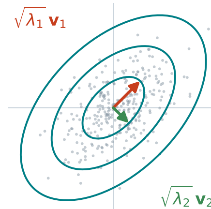
2D: \Sigma with rows (2, 1) and (1, 2)
