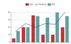
Barline Chart
