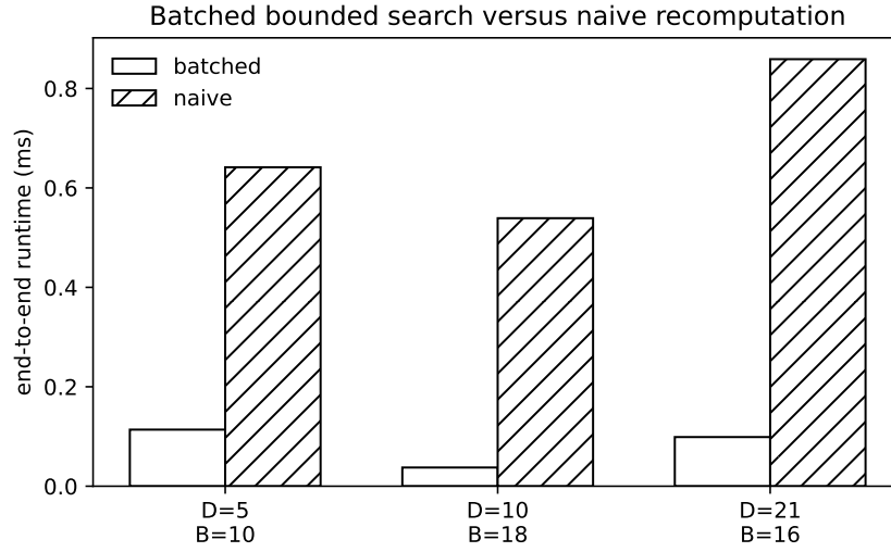
Fig. 4. End-to-end runtimes for the batched bounded routine and naive per-target recomputation in Table 7. The important comparison is the full batched end-to-end runtime versus the full naive end-to-end runtime.
