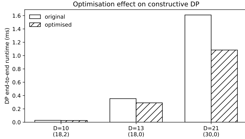
Fig. 3. End-to-end constructive DP runtimes before and after internal coefficient reordering and repeated-coefficient caching for the optimisation benchmarks of Table 6.
