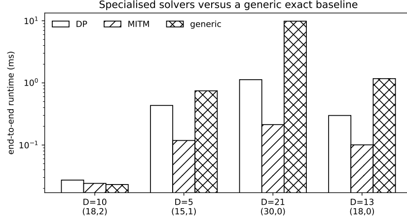
Fig. 2. End-to-end runtimes for constructive DP, meet-in-the-middle, and the bundled generic exact baseline of Table 5. The specialised solvers exploit partial-sum reuse, whereas the generic baseline expands the full Cartesian product of the value lists.
