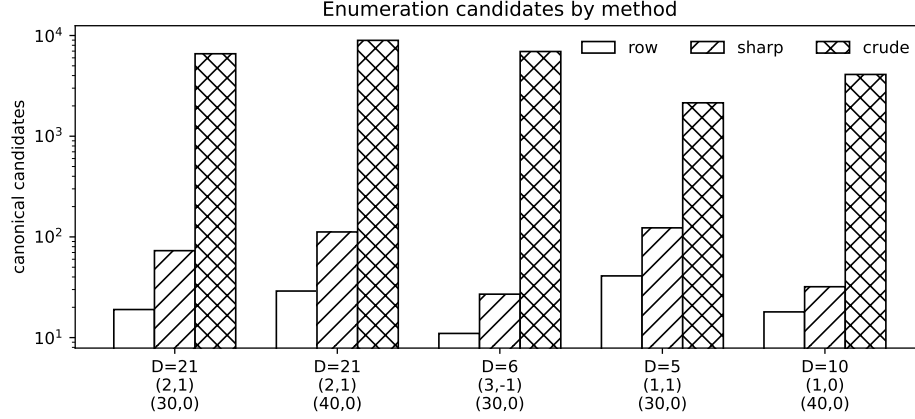
Fig. 1. Canonical candidate counts on a logarithmic scale for the weighted-search benchmarks of Table 3. The exact row search consistently stays below the sharp-box baseline and far below the deliberately crude box.
