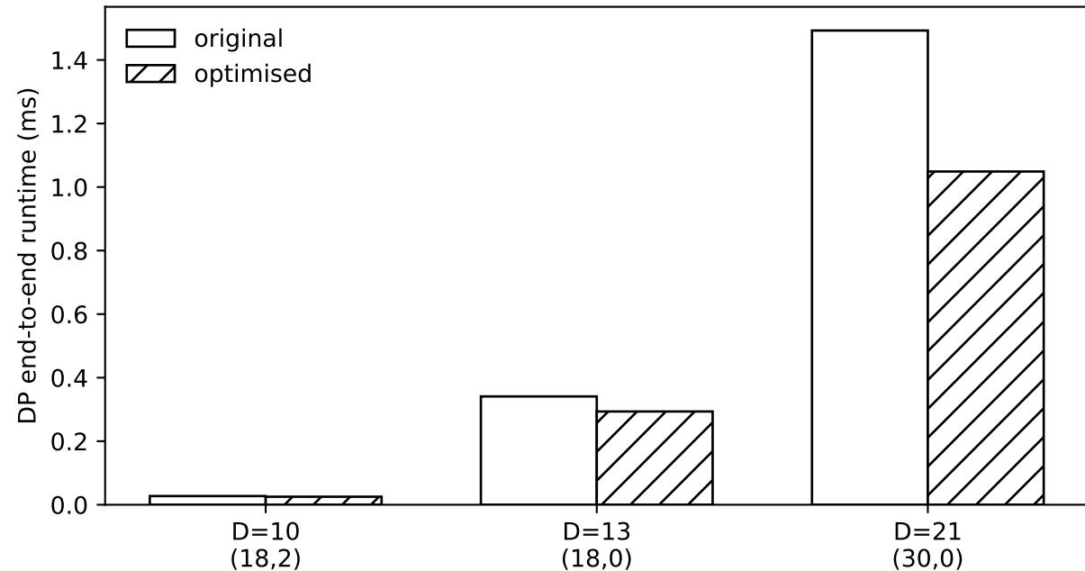
Optimisation effect on constructive DP
