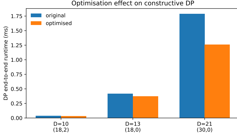
FIGURE 3. End-to-end constructive DP runtimes before and after internal coefficient reordering and repeated-coefficient caching for the optimisation benchmarks of Table 4.
