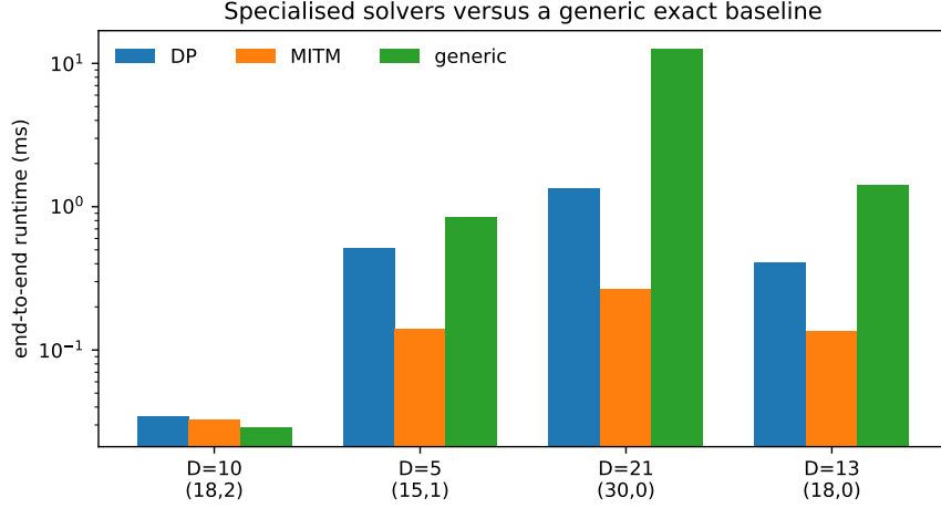
FIGURE 2. End-to-end runtimes for constructive DP, meet-in-the-middle, and the bundled generic exact baseline of Table 3. The specialised solvers exploit partial-sum reuse, whereas the generic baseline expands the full Cartesian product of the value lists.
