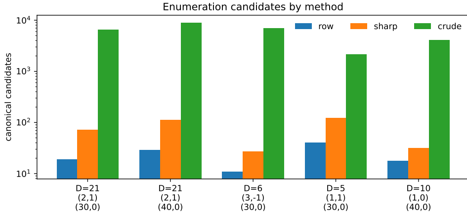
FIGURE 1. Canonical candidate counts on a logarithmic scale for the weighted-search benchmarks of Table 1. The exact row search consistently stays below the sharp-box baseline and far below the deliberately crude box.
