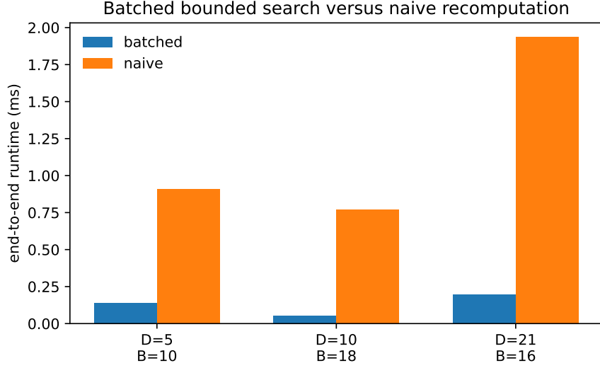
FIGURE 4. End-to-end runtimes for the batched bounded routine and naive per-target recomputation in Table 5. The important comparison is the full batched end-to-end runtime versus the full naive end-to-end runtime.
