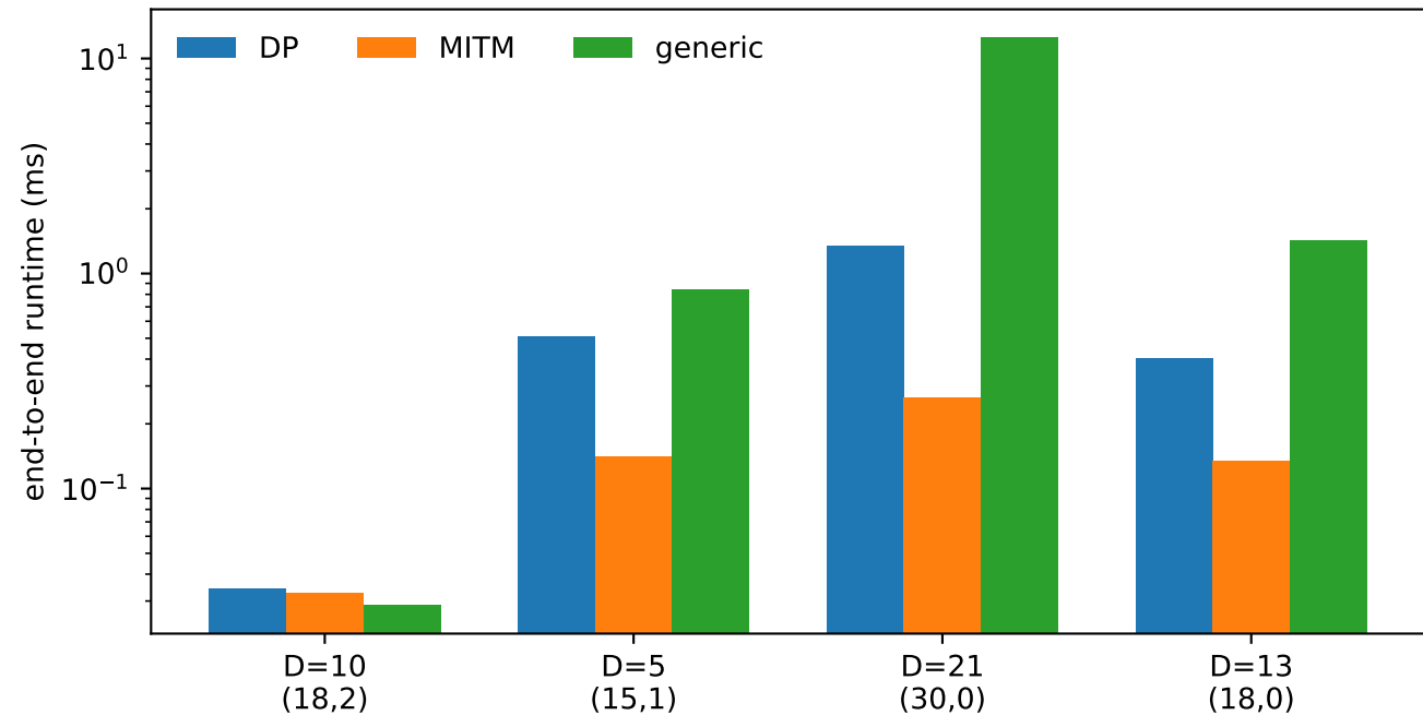
Specialised solvers versus a generic exact baseline
