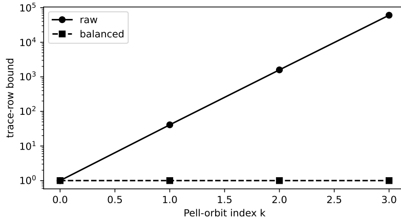
Fig. 1. Raw and balanced trace-row bounds along the Pell orbit in the balancing ablation.
