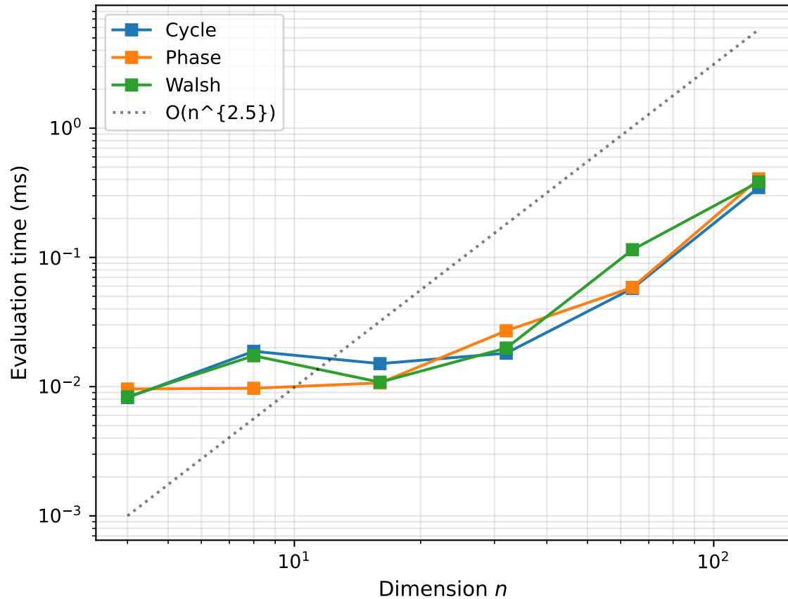
P(\Lambda) computation cost
