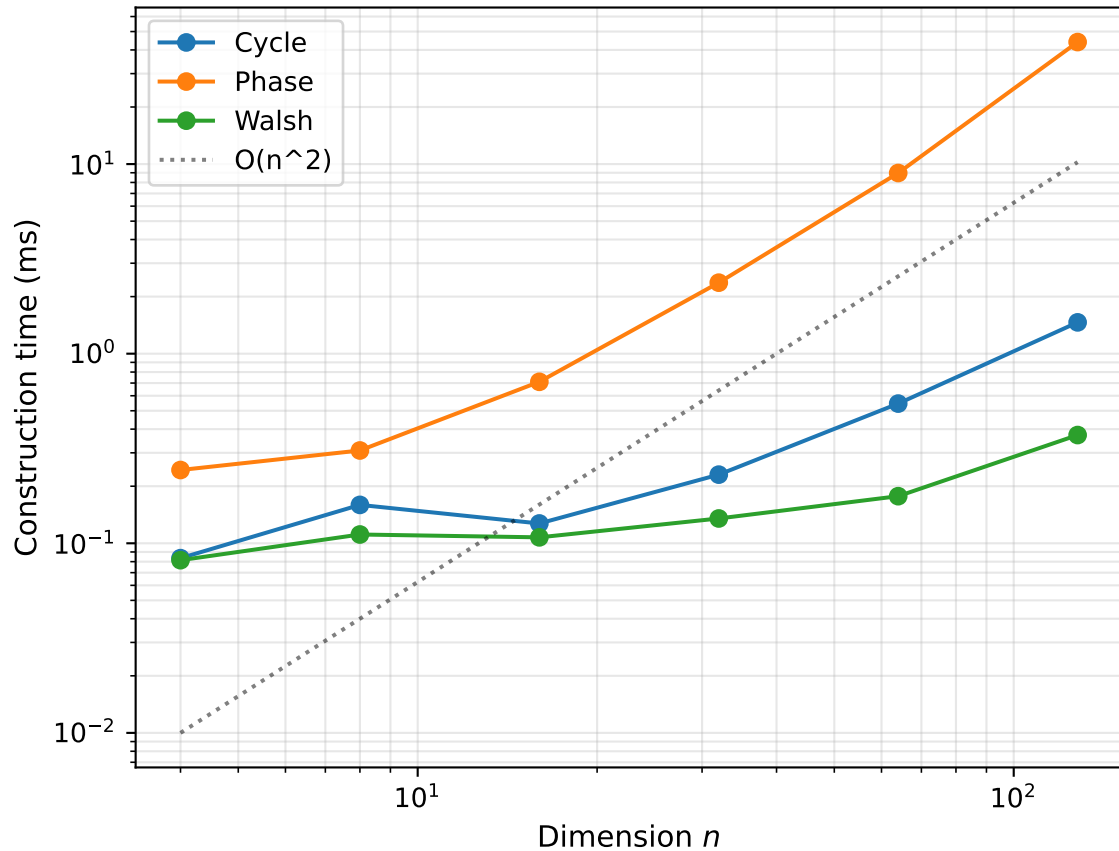
Basis construction cost
