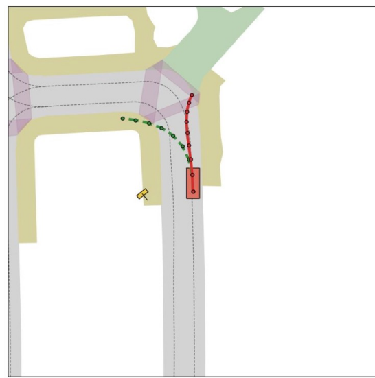
OneVL BEV
