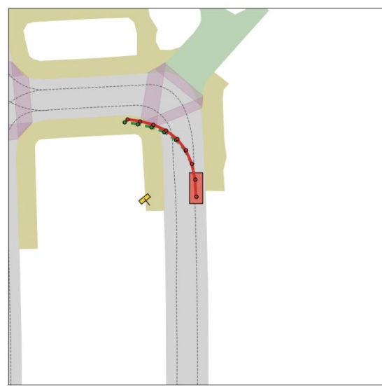
OneVL Reasoning
