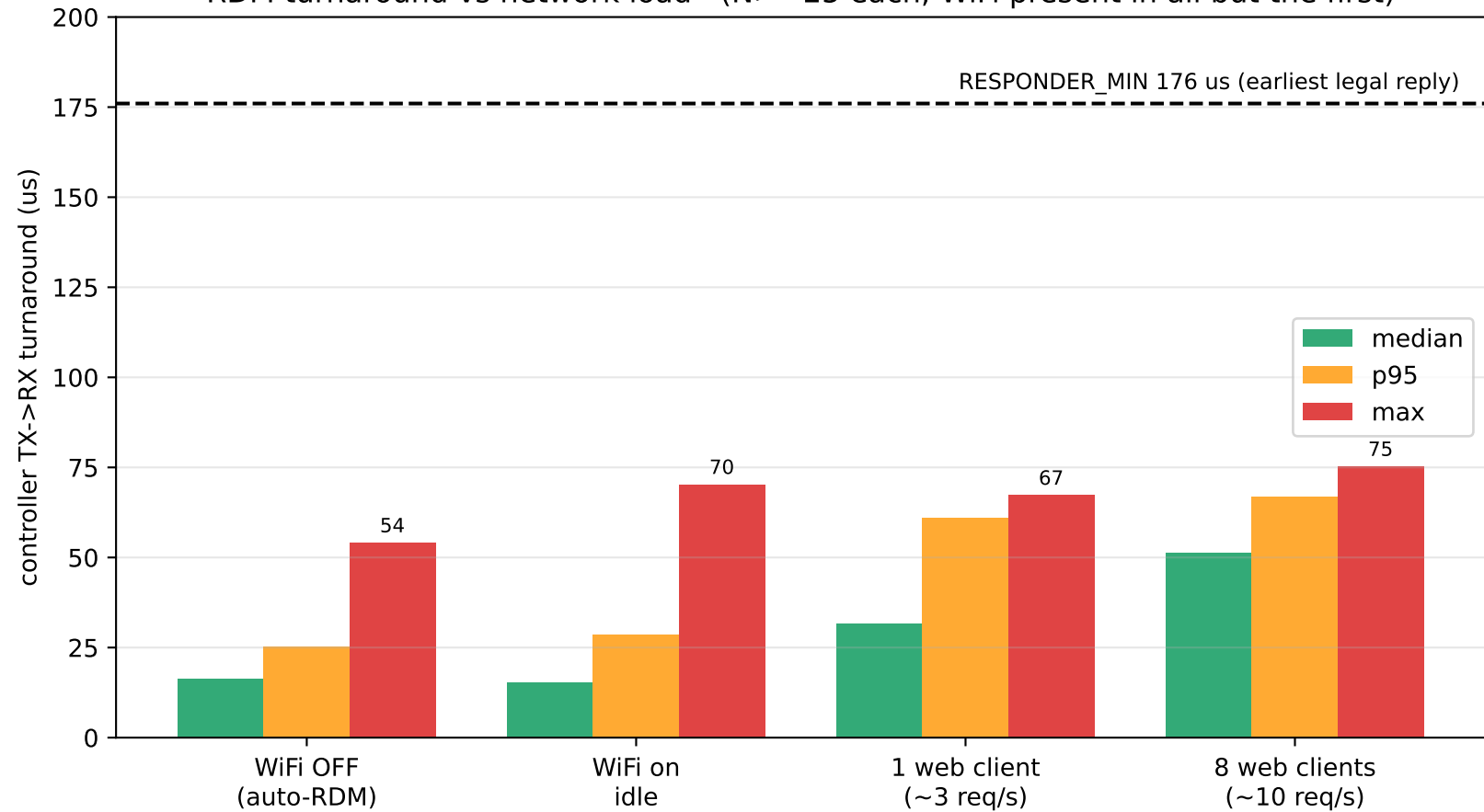
RDM turnaround vs network load (N>=25 each; WiFi present in all but the first)
