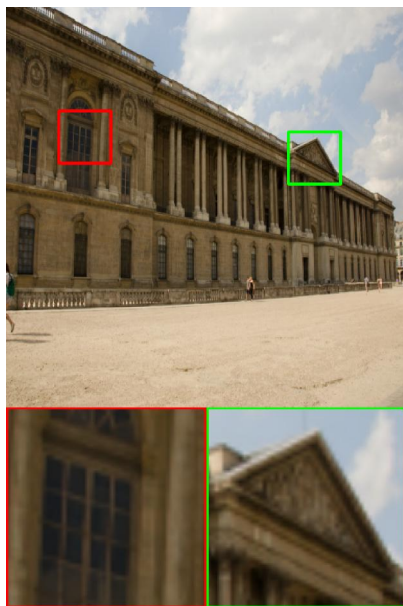
KinD
