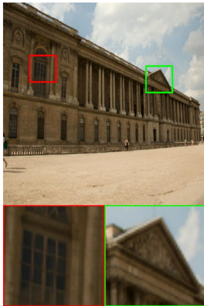
KinD
