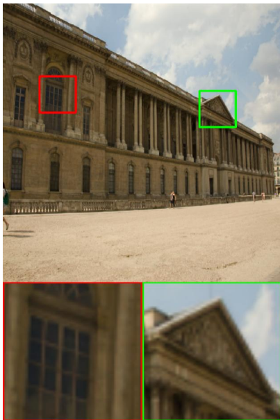
LLFormer
