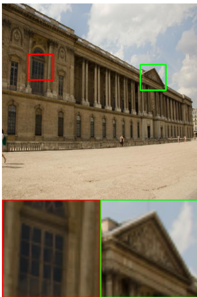
RetinexNet
