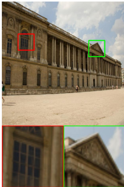
FourLLIE
