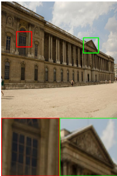
RetinexNet
