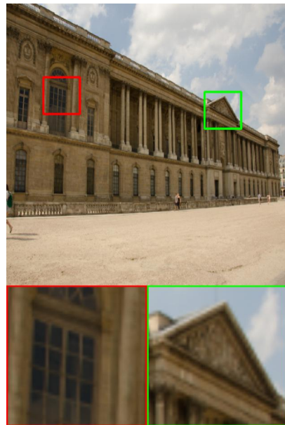
PPFormer
