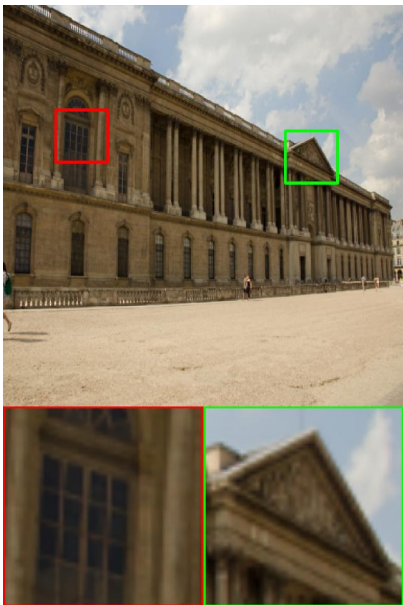
URetinex-Net
