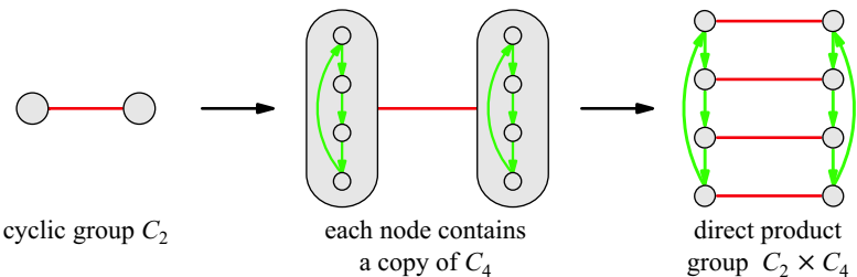
Figure 7.2. The construction of a Cayley diagram for the group C_2 \times C_4 , using Cayley diagrams of C_2 and C_4 , as described in Definition 7.1
