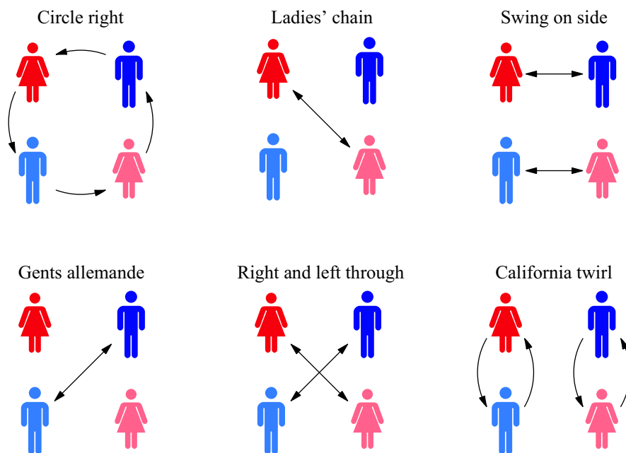
Figure 3.15. How six example contra dance figures rearrange the dancers.
