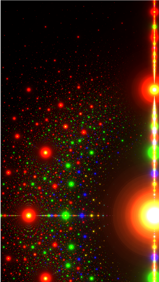
Figure: Algebraic numbers in the complex plane. Colors indicate the coefficient of the leading term: red = 1 (algebraic integer) , green = 2 , blue = 3 , yellow = 4 . Large dots mean fewer terms and smaller coefficients. Image from Wikipedia (made by Stephen J. Brooks).
