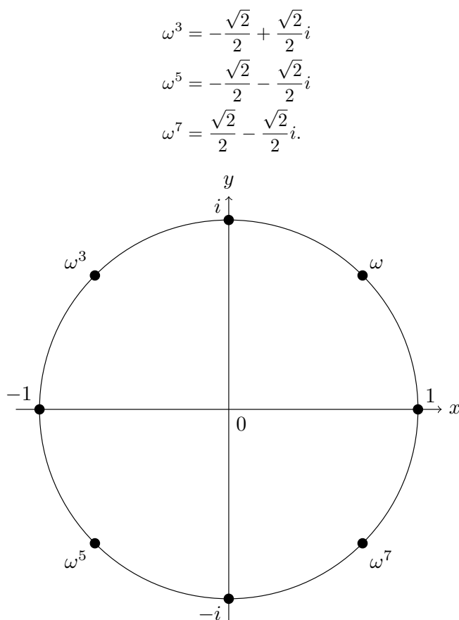
Figure 4.27 8th roots of unity
