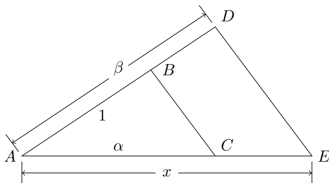
Lemma 21.39 If \alpha is a constructible number, then \sqrt{\alpha} is a constructible number.
