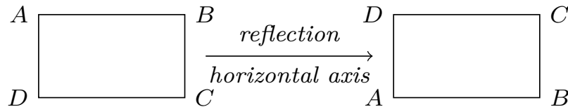
Figure 3.5 Rigid motions of a rectangle
