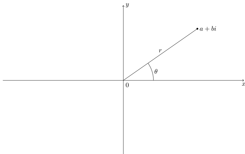
Figure 4.18 Polar coordinates of a complex number
