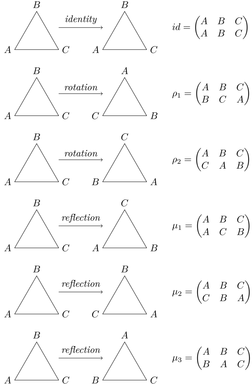
Figure 3.6 Symmetries of a triangle
