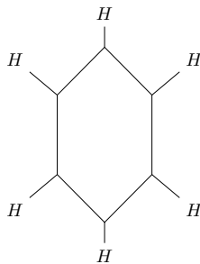
Figure 14.28 A benzene ring
