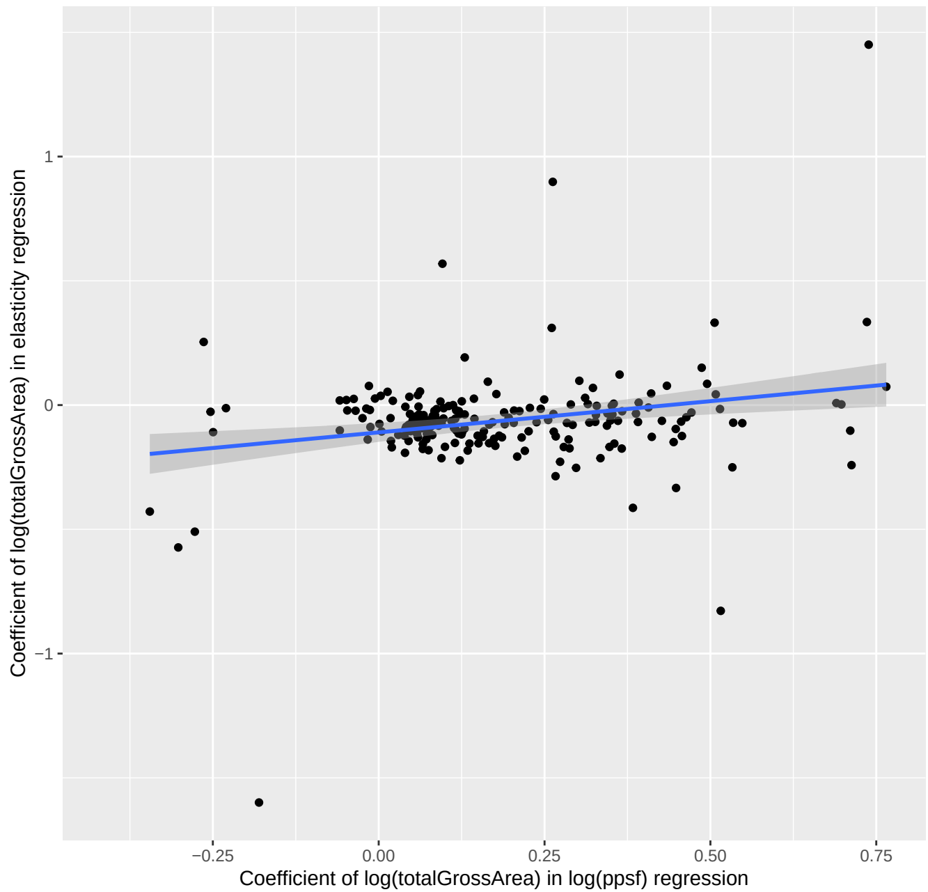
Relationship between price per square foot and elasticity of price per square foot v
