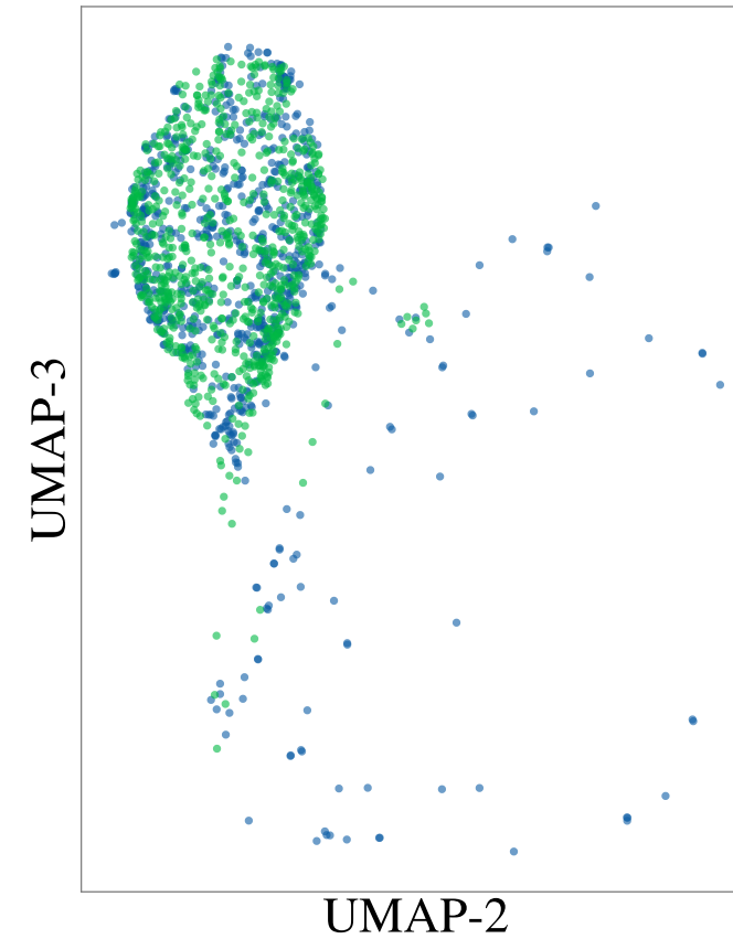
Fast Scattering
