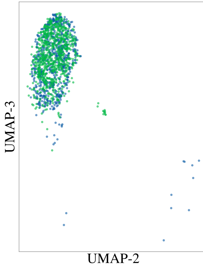
Scattered Light
