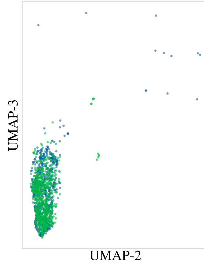
Scattered Light
