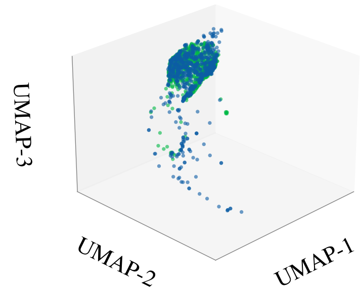
Fast Scattering
