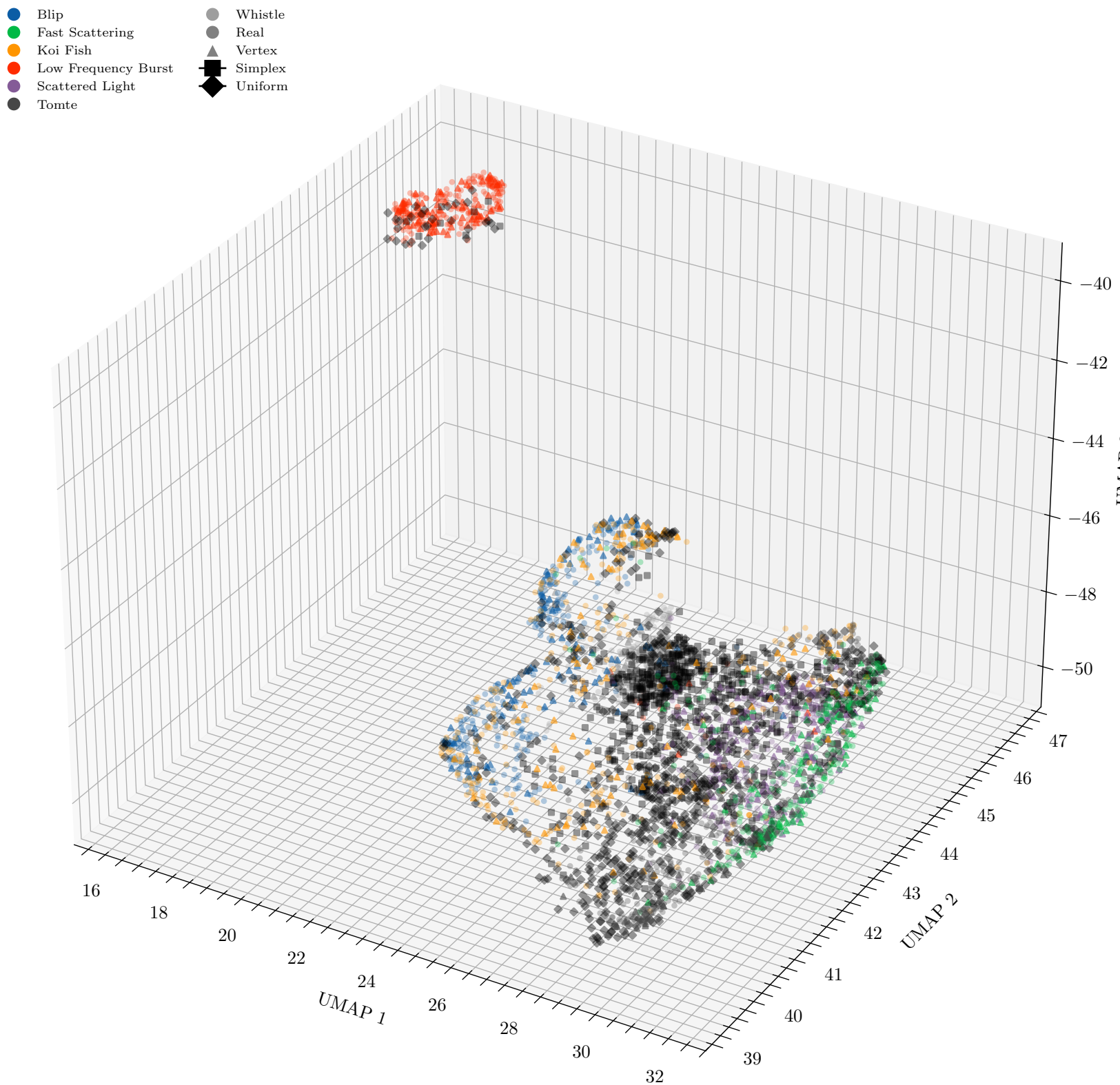
3D UMAP: sampling modes (epoch 210)
