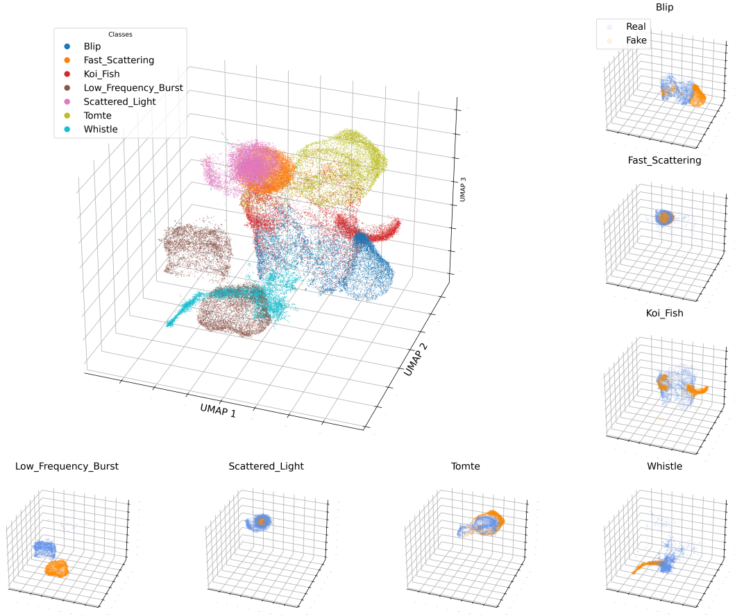
FIG. 12: Three-dimensional UMAP projection of real (orange) and DiT-generated (blue) glitches across all seven classes. The large panel shows the overall structure, while smaller panels display each class individually. Overlapping clusters indicate morphological similarity between real and synthetic samples; separable clusters for most classes indicate that DiT does not reproduce the full morphological structure of real glitches, in contrast to GlitchGAN (Figure 5).
