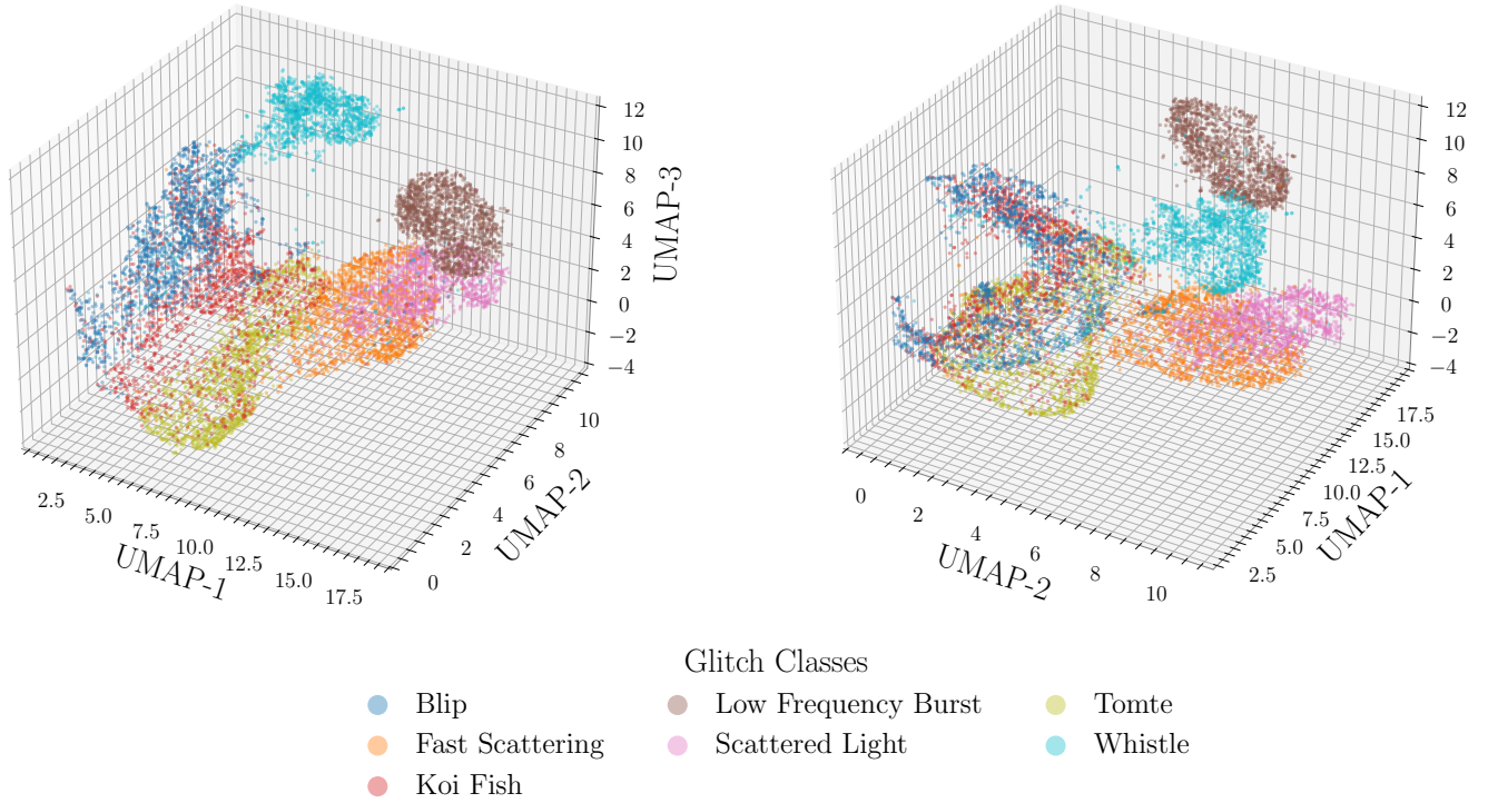
FIG. 5: Two complementary views of three-dimensional UMAP embeddings showing real and generated glitch samples. Each color corresponds to one of the seven glitch classes used during training.
