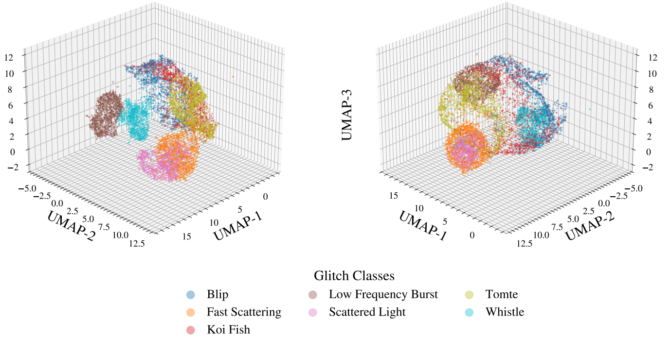
FIG. 5: Two complementary views of three-dimensional UMAP embeddings showing real and generated glitch samples. Each color corresponds to one of the seven glitch classes used during training.
