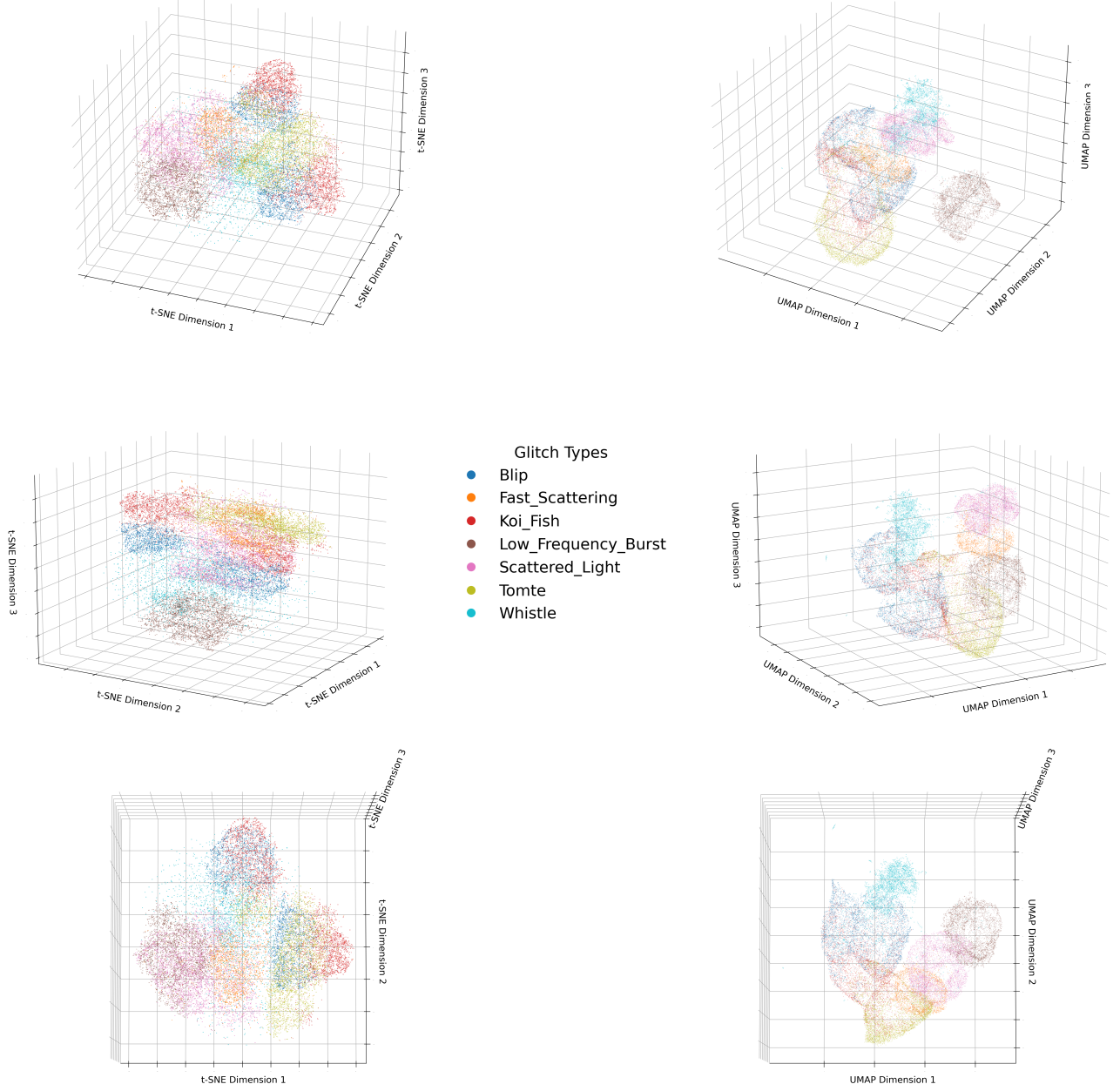
FIG. 3: Three-dimensional t -SNE (left) and UMAP (right) embeddings of DeepExtractor reconstructions across three viewpoints. Colours correspond to Gravity Spy glitch classes. Well-separated clusters demonstrate that reconstructions preserve class-specific morphological structure in the time domain. The partial overlap between Blip and Koi Fish (visible in the middle row) is consistent with their known morphological proximity.
