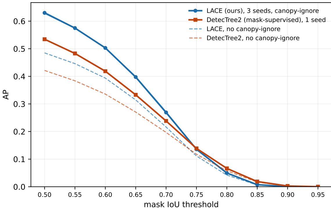
OAM-TCD 439: AP across IoU thresholds
