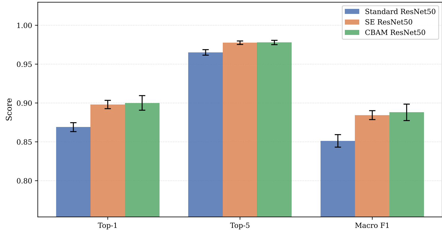
Phase 1 — CompCars: Mean Scores ( \pm 1 std, 10 folds)
