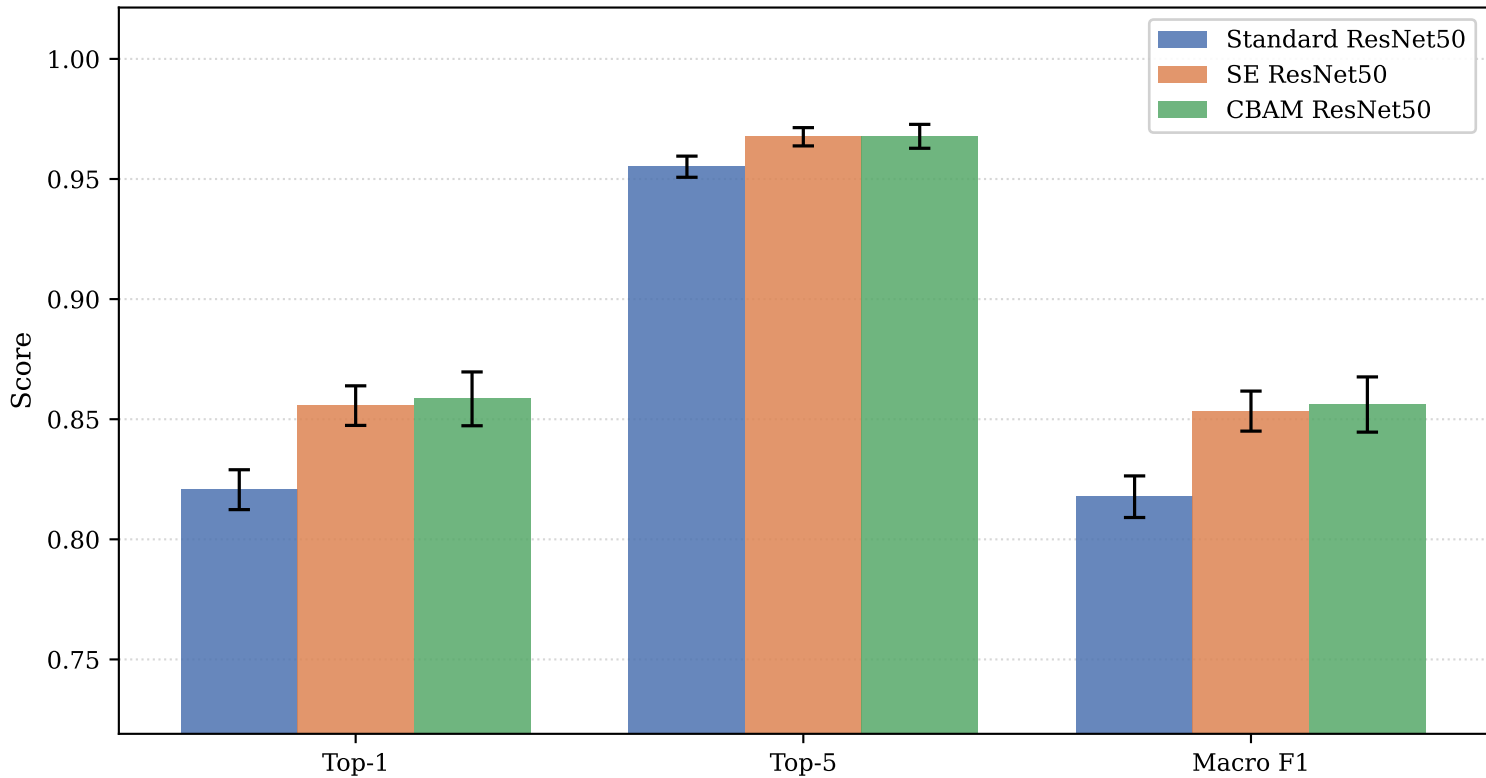
Phase 1 — Stanford Cars: Mean Scores ( \pm 1 std, 10 folds)
