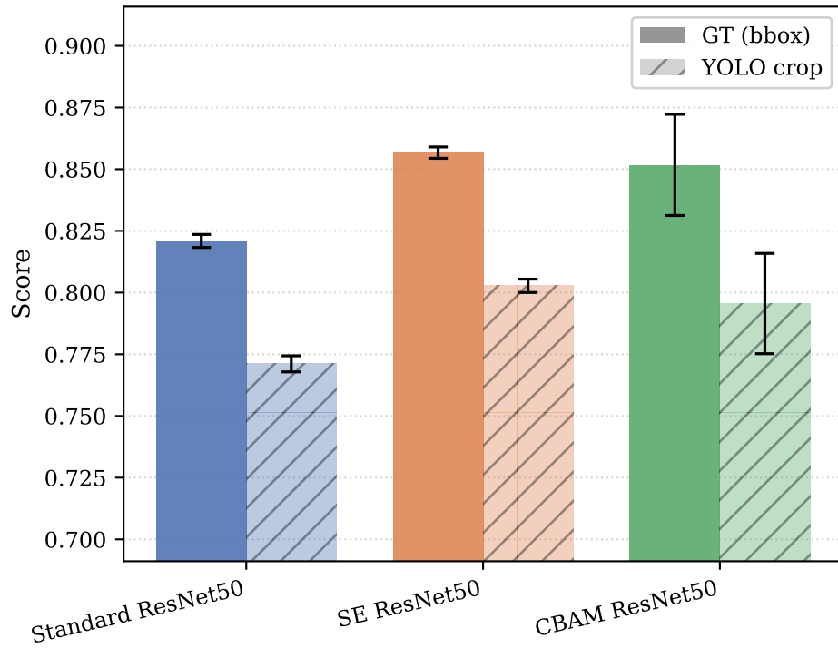
Top-1 Accuracy
