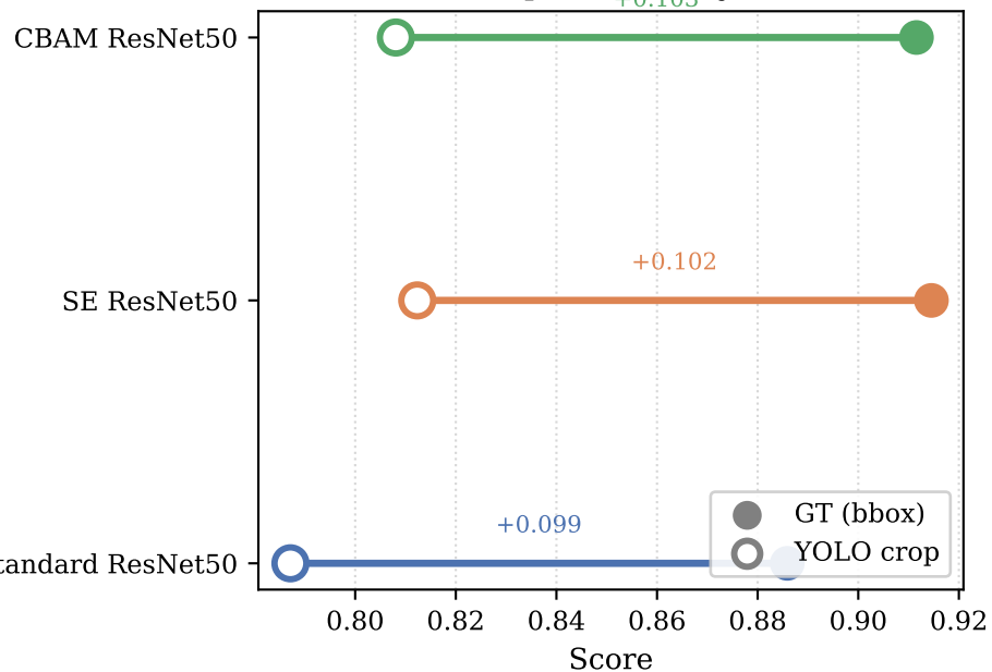
Top-1 Accuracy
