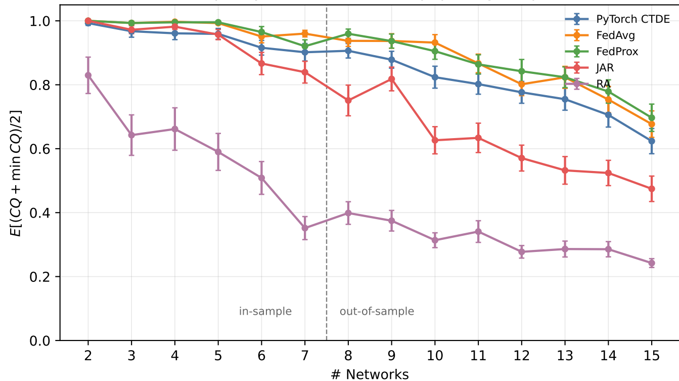
Channel quality vs network count (paper Fig. 13 protocol)
