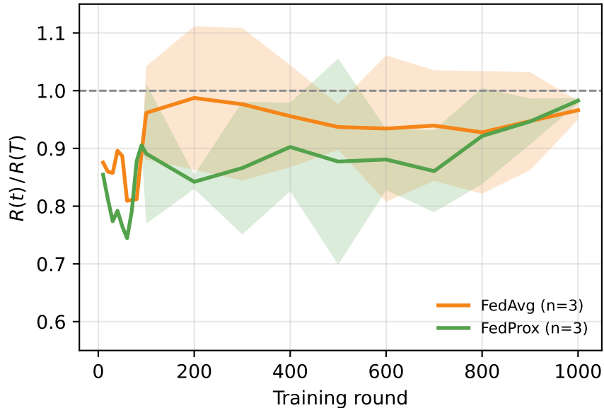
(b) Normalized learning curve
