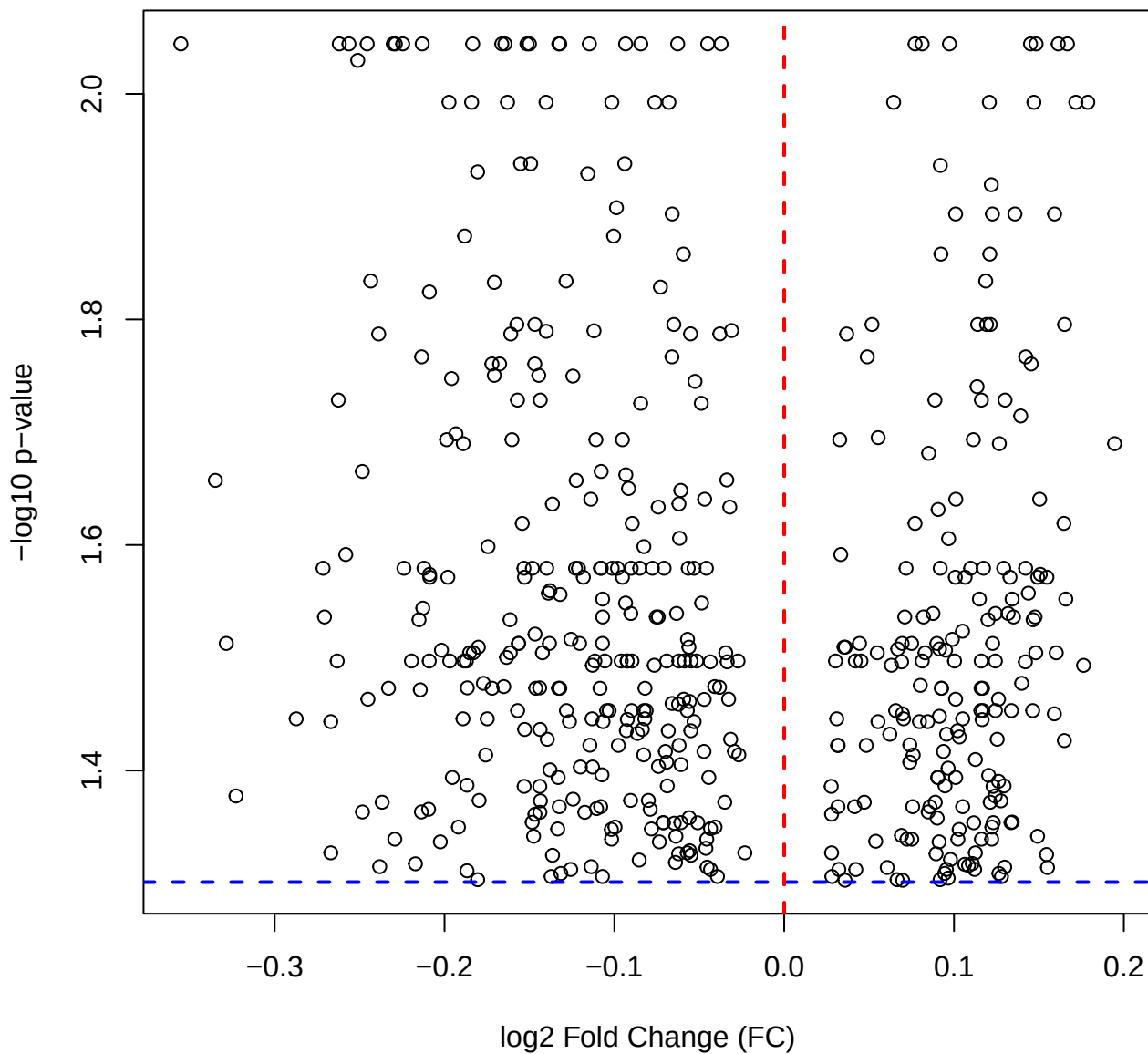
Volcano plot after filtering
