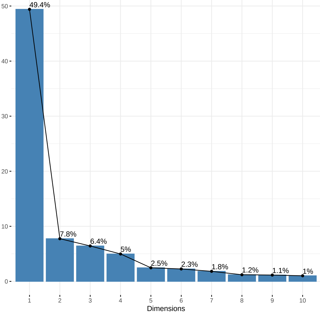
Scree plot
