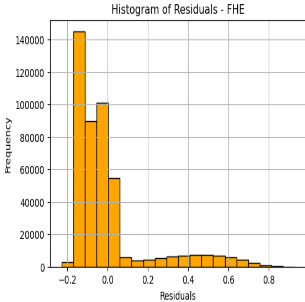
Residual Histogram - Test
