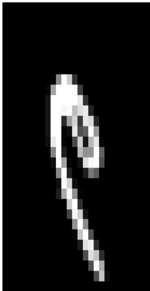
Predicted: 9
