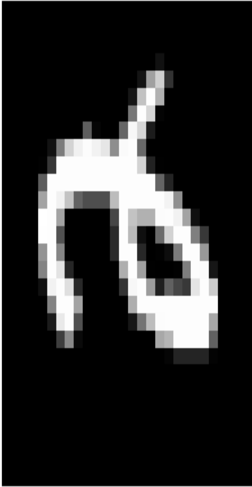
Ground Truth: 2
