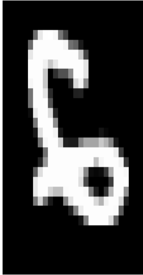
Predicted: 2
