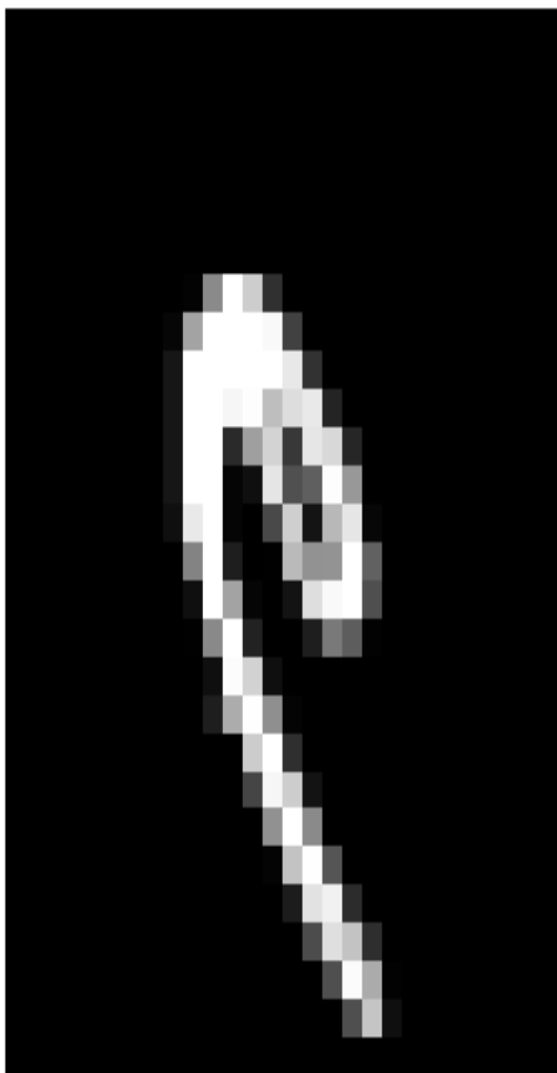
Ground Truth: 9
