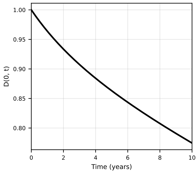
Discount factor D(0, t)
