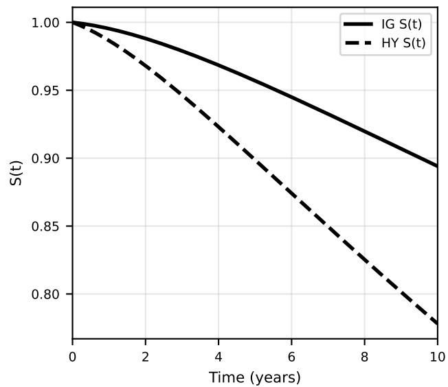
Survival probability S(t)
