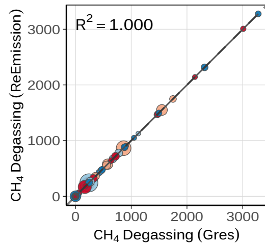
CH 4 Degassing
