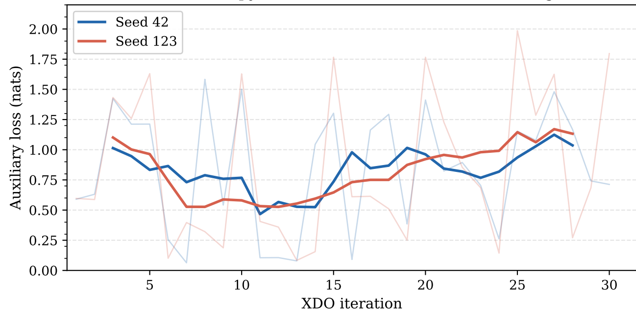
Auxiliary Partner-Prediction Loss per XDO Iteration (cross-entropy; lower = better convention encoding)
