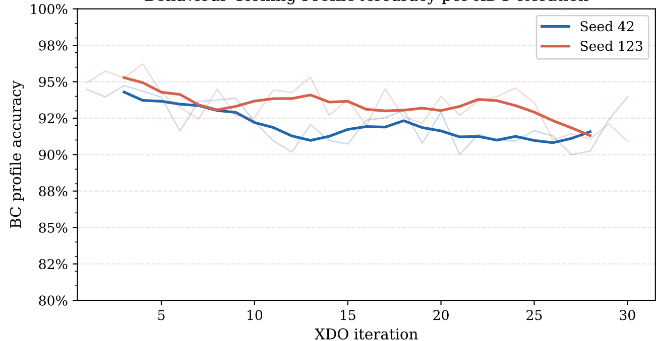
Behaviour Cloning Profile Accuracy per XDO Iteration
