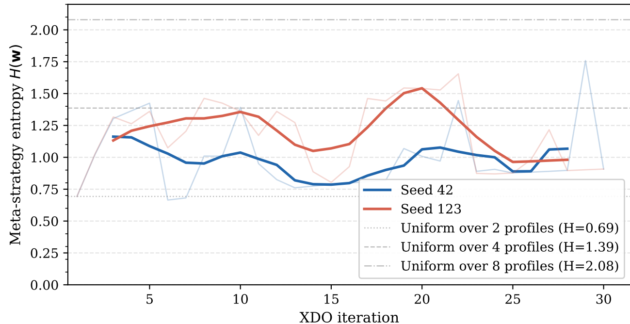
Meta-Strategy Entropy ( \alpha = 0.5 )
