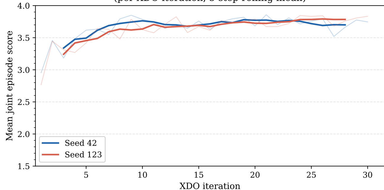
Greedy Evaluation Rollout Score (per XDO iteration, 5-step rolling mean)
